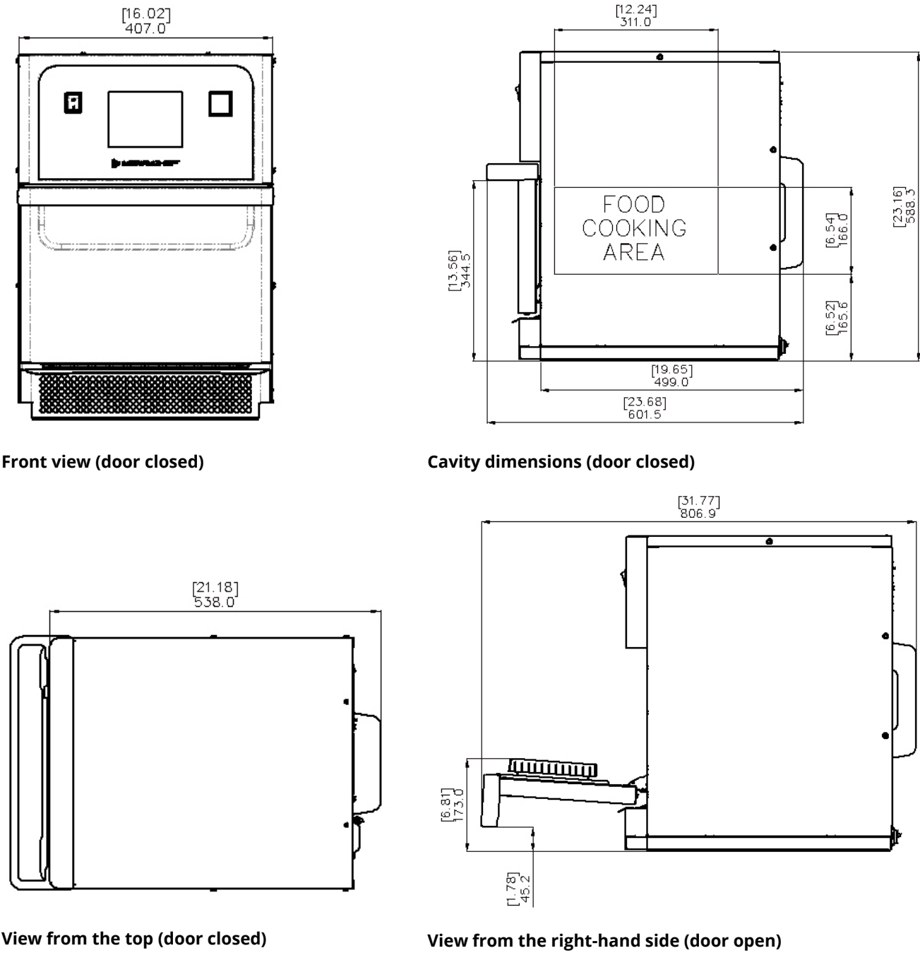
Figure 3.5: e1s dimensions with doors open and closed
