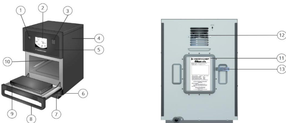
Figure 3.2: e1s front and rear views – parts and safety devices
