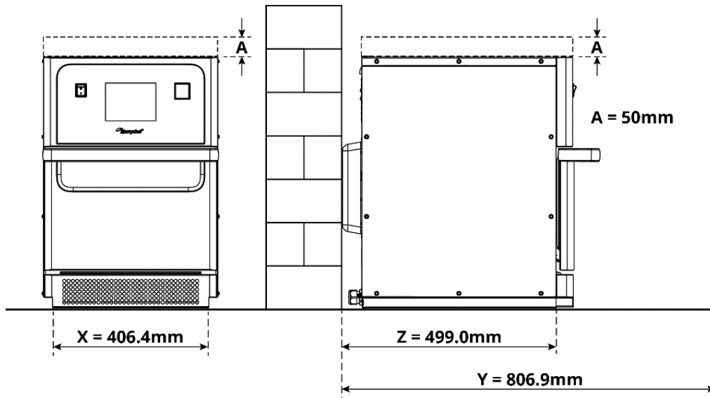
Figure 3.4: Minimum space requirements
